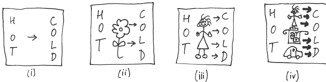
FIG. 1. Evolution of species and computation, driven by the second law of thermodynamics (as inspired by England’s et al approach [8, 9]): (i) interface between hot and cold regions is empty space; (ii) plant interface capable of more dissipation than empty space; (iii) animals and, in particular, humans (drawn political correctly) present interfaces with improved (over plants and emptiness) energy dissipation; (iv) humans with engines and universal computation capacities (indicated by “T” for “universal Turing machine”) can consume even more energy than standalone.
