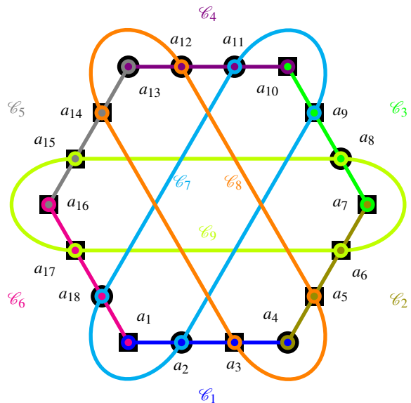
FIG. 2. Orthogonality diagram (hypergraph) of a configuration of observables without any two-valued state, used in a parity proof of the Kochen-Specker theorem presented by Cabello, Estebaranz-García-Alcaine [6]. One (from 9216) underlaid value assignments represents squares as “+1” and circles as “-1”. A quantum realization is, for example, in terms of 18 orthogonal projection operators associated with the one dimensional subspaces spanned by the vectors from the origin (0,0,0,0)^T to |a_1\rangle = (0,0,1,-1)^T , |a_2\rangle = (1,-1,0,0)^T , |a_3\rangle = (1,1,-1,-1)^T , |a_4\rangle = (1,1,1,1)^T , |a_5\rangle = (1,-1,1,-1)^T , |a_6\rangle = (1,0,-1,0)^T , |a_7\rangle = (0,1,0,-1)^T , |a_8\rangle = (1,0,1,0)^T , |a_9\rangle = (1,1,-1,1)^T , |a_{10}\rangle = (-1,1,1,1)^T , |a_{11}\rangle = (1,1,1,-1)^T , |a_{12}\rangle = (1,0,0,1)^T , |a_{13}\rangle = (0,1,-1,0)^T , |a_{14}\rangle = (0,1,1,0)^T , |a_{15}\rangle = (0,0,0,1)^T , |a_{16}\rangle = (1,0,0,0)^T , |a_{17}\rangle = (0,1,0,0)^T , |a_{18}\rangle = (0,0,1,1)^T , respectively.
