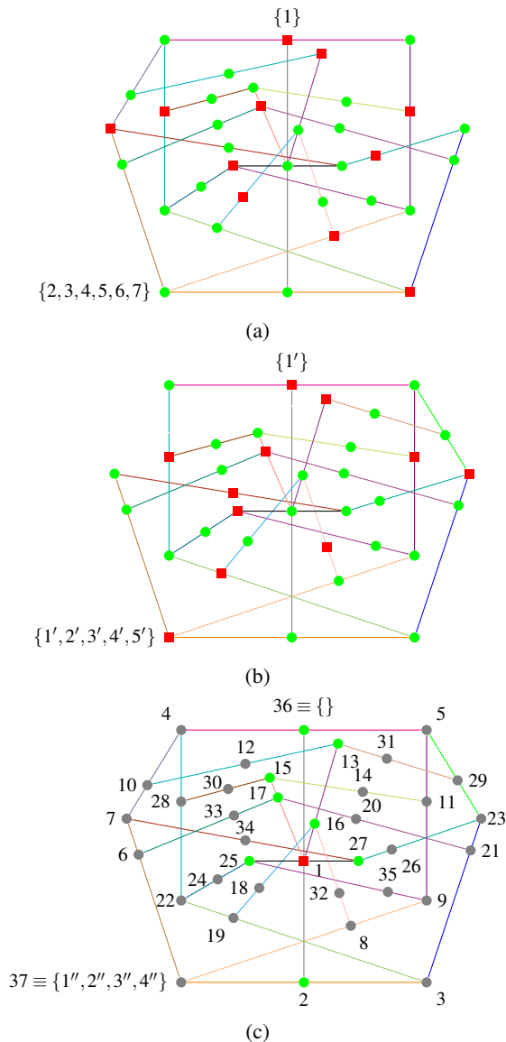
FIG. 2. (a) TIFS cloud, and (b) TITS cloud with only a single overlaid classical value assignment if the system is prepared in state |1\rangle (Svozil 2018b). (c) The combined cloud from (a) and (b) has no value assignment allowing 36 = \{\} to be true/1; but still allows 8 classical value assignments enumerated by Table I, with overlaid partial coverage common to all of them. A faithful orthogonal realization is enumerated in Ref. (Abbott et al 2015, Table. 1, p. 102201-7).
