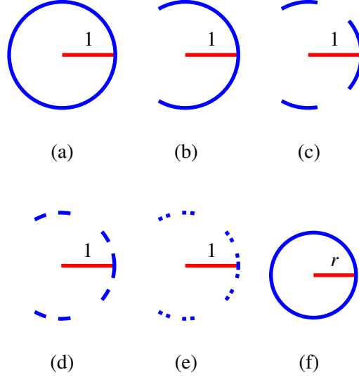
FIG. 2. A fractal example of why “cutting out holes” or “creating gaps” in a continuum in a scale invariant manner might yield different radii if the remaining pieces are scaled by the fractal dimension and subsequently “pasted” together. (a) consider an original circle with radius 1; (b) the middle third segment [\frac{2\pi}{3}, \frac{4\pi}{3}) is cut out of (a), thereby effectively reducing the length of the set by a factor of \frac{1}{3} ; (c) the middle third segments [\frac{2\pi}{9}, \frac{4\pi}{9}) and [\frac{14\pi}{9}, \frac{16\pi}{9}) are cut out of the remaining segments in (b), thereby effectively reducing the length of the set by a factor of \frac{1}{3} ; (d)–(e) shows the iteration of this construction; (f) alternatively one can draw a full circle with a pasting of the upscaled segments and a reduced radius r \approx 0.8 from Eq. (2).
