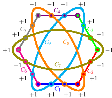
FIG. 10. (Color online) Orthogonality diagram of a finite subset C_1, \dots, C_9 of the continuum of blocks or contexts embeddable in four-dimensional real Hilbert space without a two-valued probability measure [43]; with one of the 1152 non-admissible value assignments yielding the bound seven, as derived in Ref [44]. In contrast, subclassicality would require that, within each one of the nine contexts, exactly one observable would have value “ -1 ,” and the other three observables would have the value “ +1 .”
