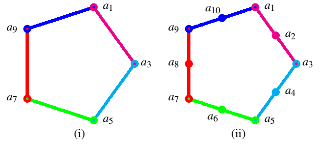
FIG. 6. (Color online) Orthogonality diagram of the reduced pentagon (i), and of the pentagon logic (ii). A realization of (ii) in terms of partition logic is enumerated in Eq. (4); an explicit quantum realization can be found in Ref. [37].
