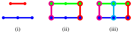
FIG. 1. (Color online) Orthogonality diagrams with mixed two- and three-atomic contexts, drawn in different colors.
