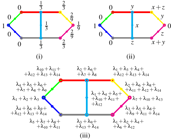
FIG. 5. (Color online) Orthogonality diagram of the logic depicted in Fig. 4 with overlaid (i) quantum and (ii) classical prediction probabilities for a state prepared along a_1 . The classical predictions require that x, y and z are non-negative and x + y + z = 1 . (iii) The full parametrization of classical probabilities; with non-negative \lambda_1, \dots, \lambda_{14} \geq 0 , and \lambda_1 + \dots + \lambda_{14} = 1 . Note that the special case (ii) is obtained by identifying with \lambda_1 = x, \lambda_2 = y, \lambda_3 = z , and \lambda_4, \dots, \lambda_{14} = 0 .
