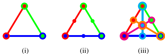
FIG. 2. (Color online) Orthogonality diagrams representing tight triangular pastings of two- and three-atomic contexts.
