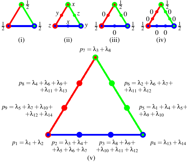
FIG. 9. (Color online) Classical probabilities (i) and (ii) of the tight triangular pastings of two- and three-atomic contexts introduced in Figs. 9(i),(ii); with x, y, z \geq 0 , and x + y + z = 1 . The prediction probabilities represented by (iii) as well as (iv) are neither classical nor quantum mechanical. The classical probabilities on the triangle logic with four atoms per context are enumerated in (v); again \lambda_1, \dots, \lambda_{14} \geq 0 and again \lambda_1 + \dots + \lambda_{14} = 1 .
