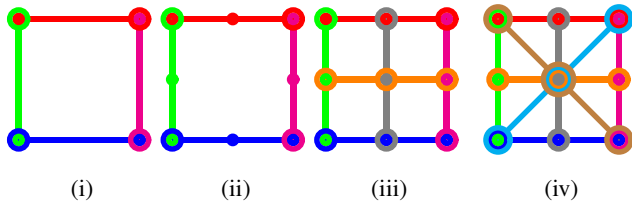
FIG. 3. (Color online) Orthogonality diagrams representing tight square type pastings of two- and three-atomic contexts.
