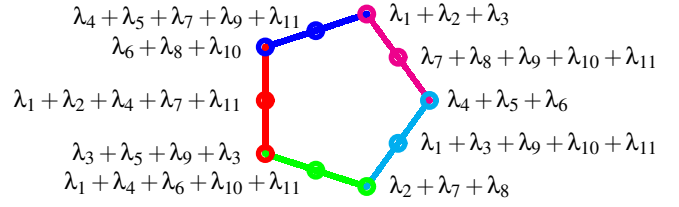
FIG. 8. (Color online) Classical probabilities on the pentagon logic.
