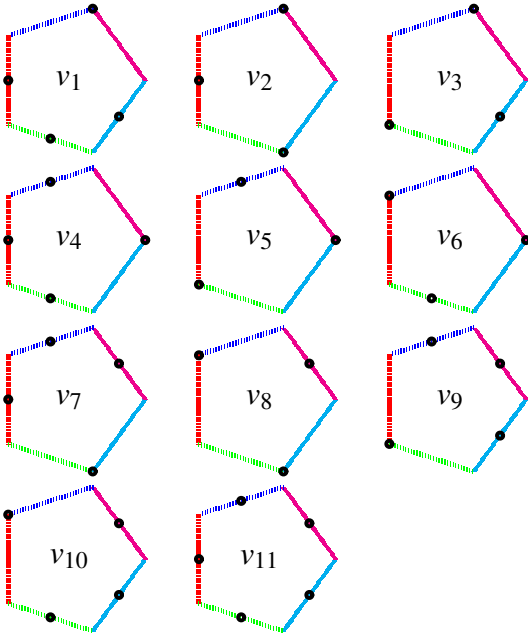
FIG. 7. Two-valued measures on the pentagon logic of Fig. 6.
