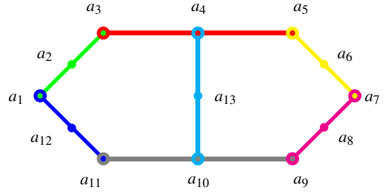
FIG. 4. (Color online) Orthogonality diagram of a cat's cradle logic which requires that, for two-valued measures, if v(a_1) = 1 , then v(a_7) = 0 . For a partition logic as well as for a Hilbert space realization see Refs. [6, 37].
