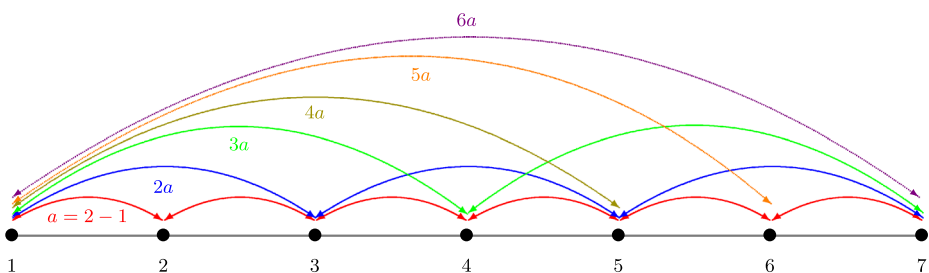
Fig. 2 (Color online) Speculative multiple side hopping might give rise to higher harmonics of the speed of light
