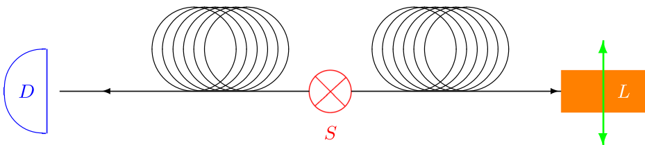
Fig. 1 (Color online) Speculative delayed choice experiment evoking stimulated emission-absorption of a quantum constituent in an entangled state. A singlet state of two quanta is created at source S . One of the particle impinges on a detector D , the other in a “box region” L filled with certain attainable quantum states
