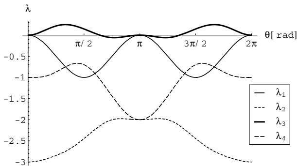
FIG. 1. Eigenvalues of O_{33} in dependence of the relative angle \theta .
