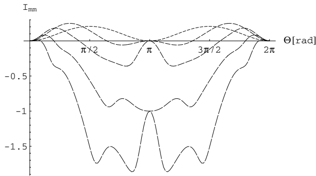
FIG. 2. Maximum violation of the operator O_{mm} for m = 2, \dots, 6 for a symmetric measurement setup; the longer dashes indicate larger m .
