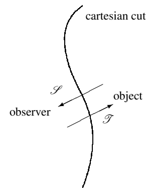
FIG. 1. An interface as a cartesian cut between observer and object. The information flow across the interface is formalized by symbols.
