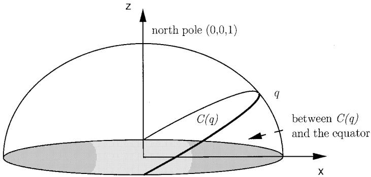
Fig. 2. The great circle C(q) .
